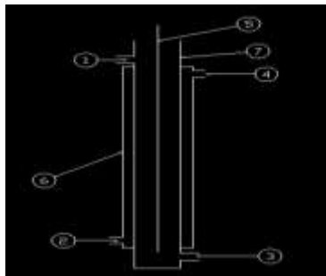
Heat transfer electric precipitator structure schematic diagram
