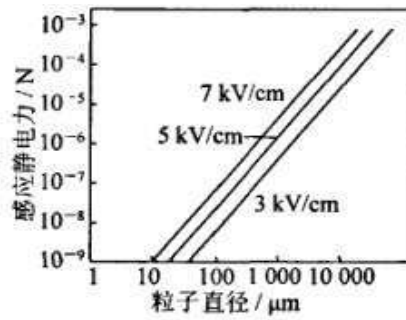
Figure 5 The relationship of induction electrostatic force, the particle diameter and ppliedvoltage
