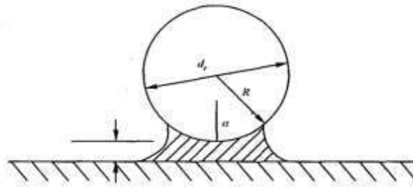
Figure 3 capillary force diagram
